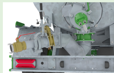
Suction/drain valve , quick coupling for Ø 150 mm hoses or fire hose couplings.
