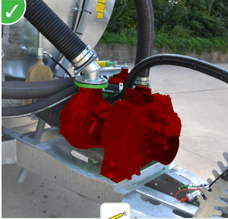
Garda/Julia Pump: vacuum pump (pumping) combined with a centrifugal pump (spraying - 6 bar)
