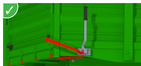
Adjustable locking system with a very large number of hooks on the side and rear drop sides to ensure a correct pressure on the seals.
