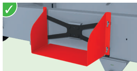
Spout for grain chute (440x240 mm) with storage under the body.
