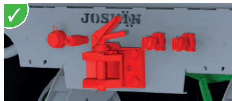
Complete connections for the lighting, braking and tipping system of a second trailer with swivel rear hitch.
