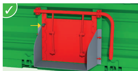
Large grain chute (opening: 390x300 mm) with automatic locking.
