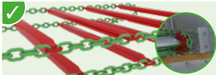
✓ Closed tubular slats welded to Ø 14 mm shipping chains (to avoid material storage) + moulded gearwheels.
