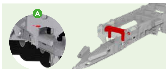
Hydropneumatic suspension drawbar on triple-axle models (optional on double-axle models).
