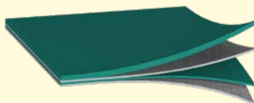
Conveyor belt structure: 4 layers of fabric and PVC with nylon reinforcement, the bottom layer being more resistant to friction.
