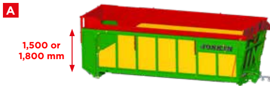
4-position mechanical extensions (50 - 250 - 400 - 550 mm), with individual adjustment on all 4 sides.
