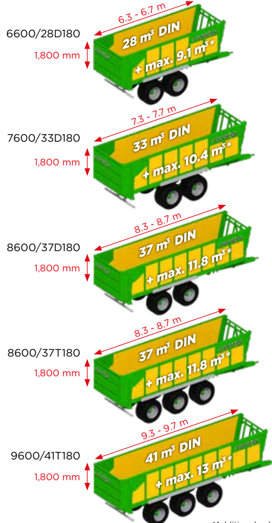
Tapered body with identical front (2,340 mm) and rear (2,380 mm) inside widths for all models.
