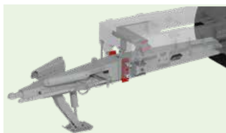
Steel drawbar guide for front suspension , with greasing points and adjustable by 4 pressure screws.
