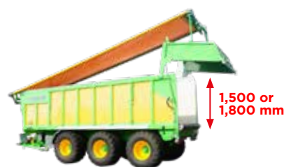
TELECOVER (hermetic) , with a single 250 mm fixed extension on the right side.
