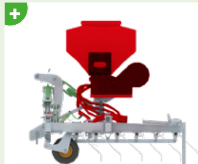
Air seeder with electric or hydraulic drive (120 or 300 l). Mounted close to the tractor for a good load distribution. Pre-equipment possible on models 480, 600, 720 and 960.
