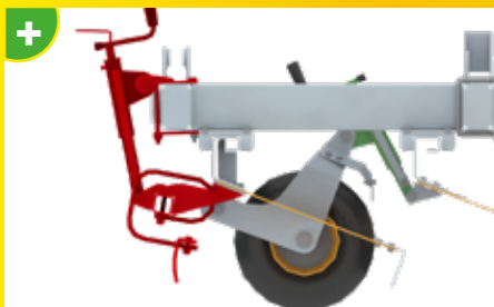
Height adjustment of the scraper blades by crank handle with graduation and marking arrow.
