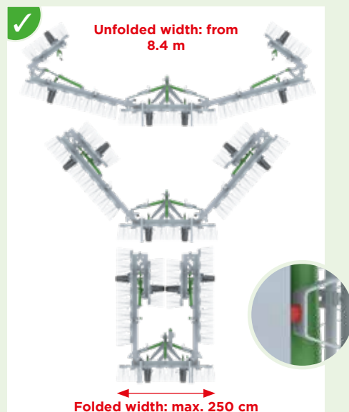
Double hydraulic folding system with adjustable stop and anti-noise Ertalon for models from 8.4 m working width.
