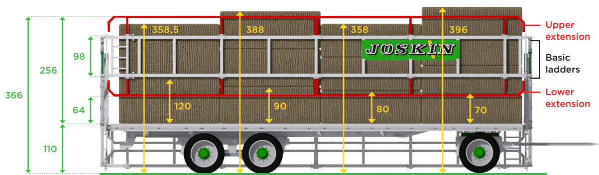
Approximate heights in cm, variable according to the wheel type.
