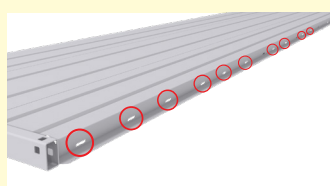
Galvanised WAGO and WAGO-Loader Lashing points
