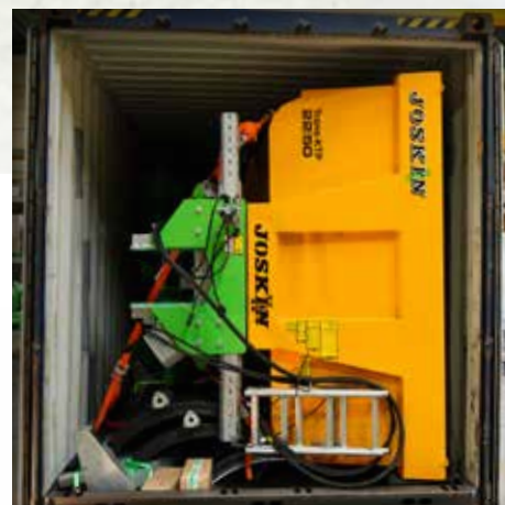
2x KTP 22/50 tipping trailer in one 40 ft HC container
